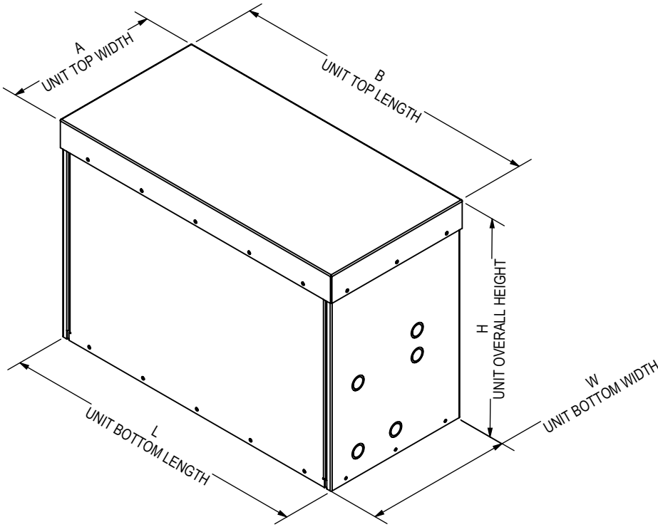
ISOMETRIC DETAIL
